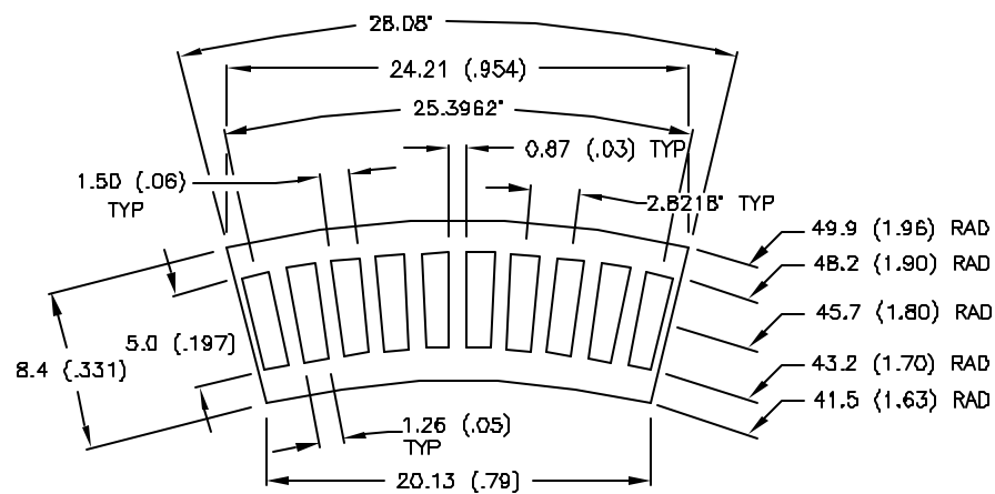
FRONT VIEW
