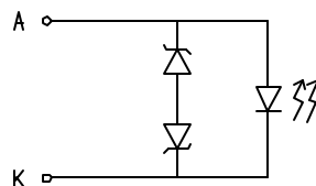
LED CIRCUIT DIAGRAM
