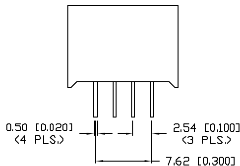
PIN OUT
