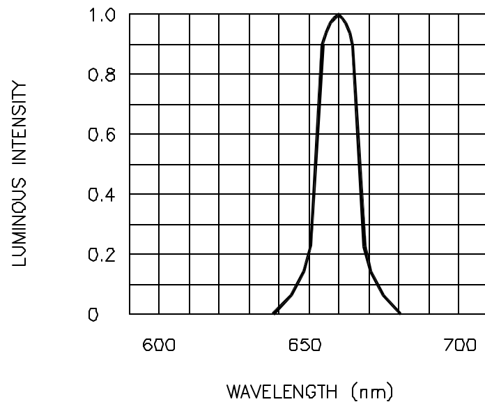
LUMINOUS INTENSITY vs WAVELENGTH
