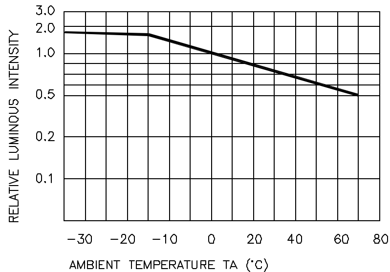
RELATIVE LUMINOUS INTENSITY vs AMBIENT TEMPERATURE
