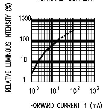
RELATIVE INTENSITY VS. FORWARD CURRENT
