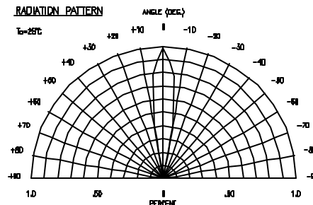
RADIATION PATTERN
