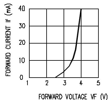
FORWARD VOLTAGE VS. FORWARD CURRENT
