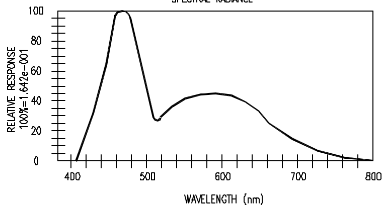
SPECTRAL RADIANCE
