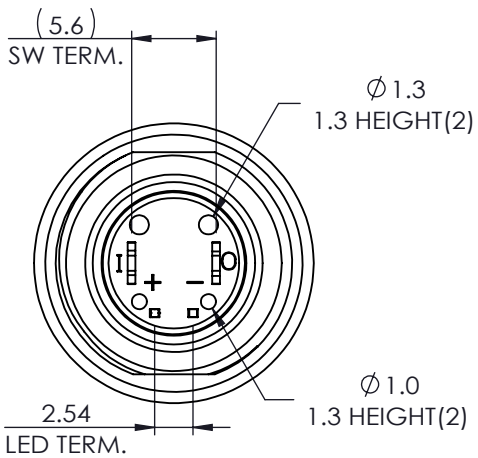
DETAIL FOR TERMINAL POSITION
