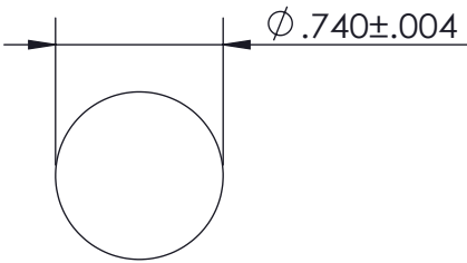
RECOMMENDED PANEL CUT-OUT MOUNT
